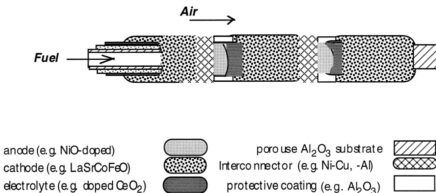
Fig. 5. Single tubular integrated fuel cell device/stack.
